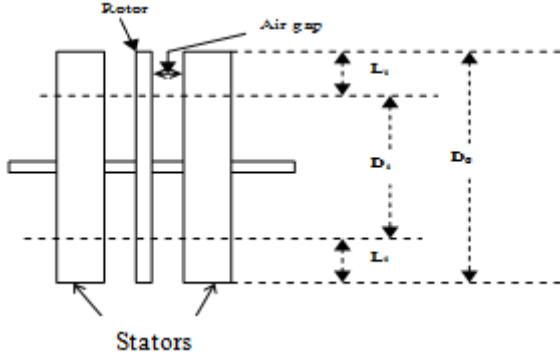
Fig.1 Simplified representation of an AFPM machine
