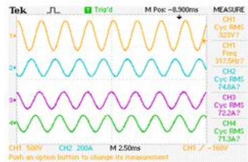
Fig.12 Voltage and current waveform at full load
