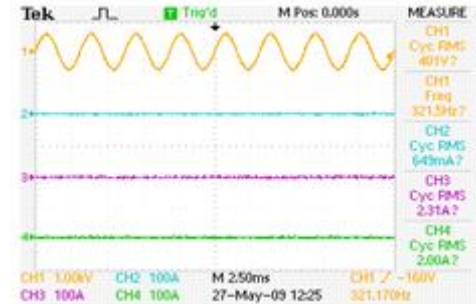
Fig.11 Voltage and current waveform at no load
